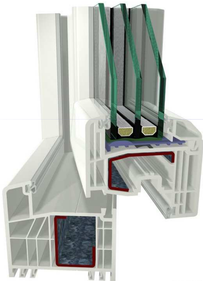
GEALAN S 8000IQ+
