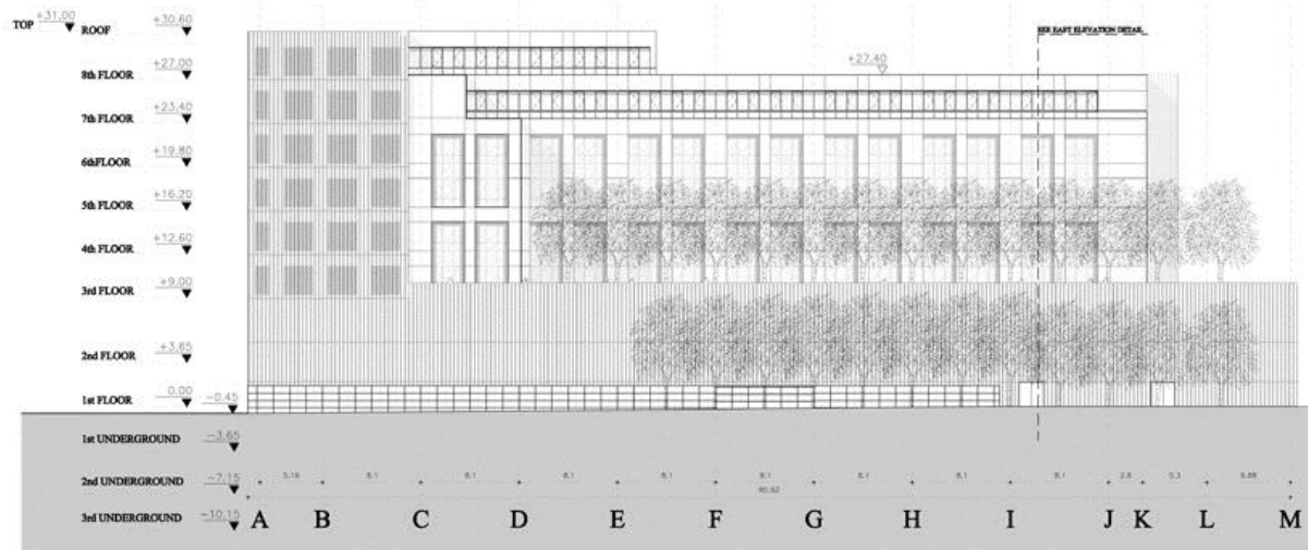
EASTERN ELEVATION SCALE: 1/200
