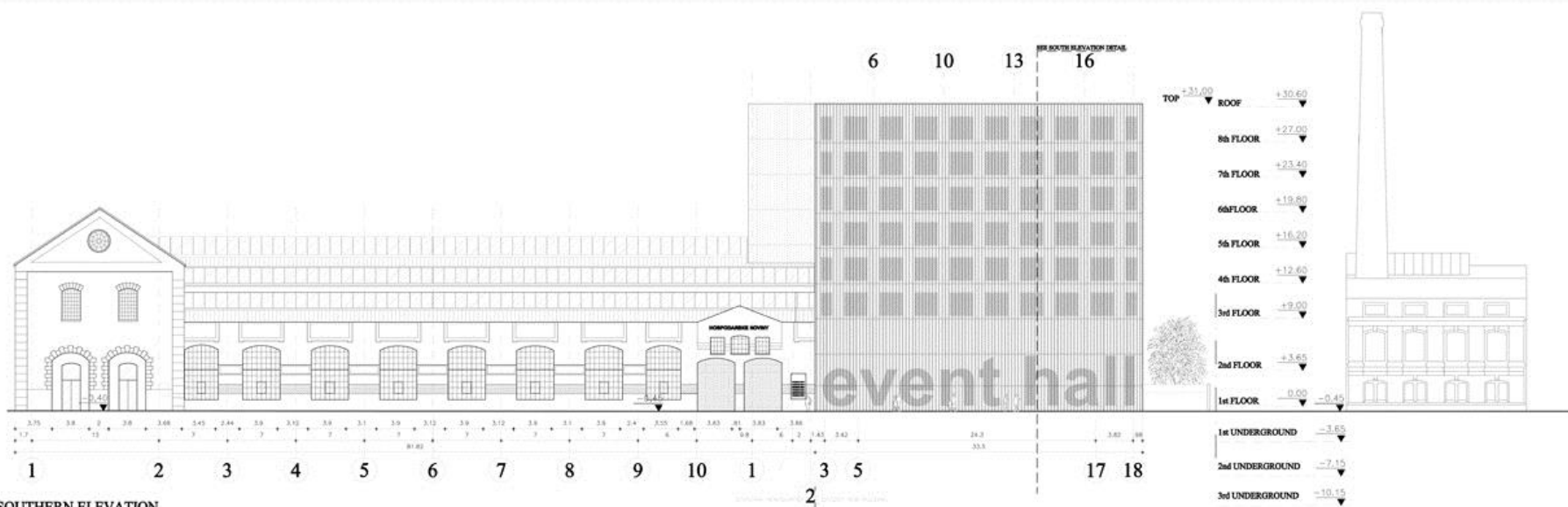
SOUTHERN ELEVATION SCALE: 1/200
